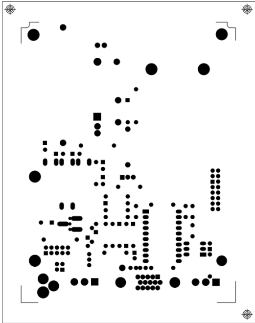
SOLDERMASK BOTTOM SIDE LS-232 PCB
