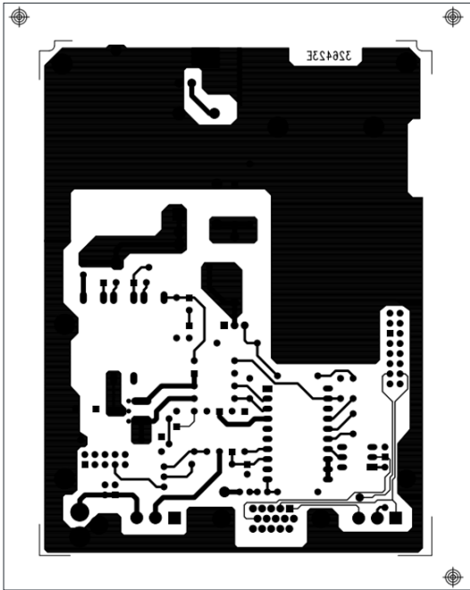
ARTWORK BOTTOM SIDE LS-232 PCB
